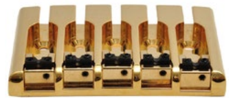
HW55G 3-D Bass Bridge, 5-String , gold, single coil. Diecasted like a Badass bridge. Steel lockable saddle. Great sound! String spacing 16.8mm.
